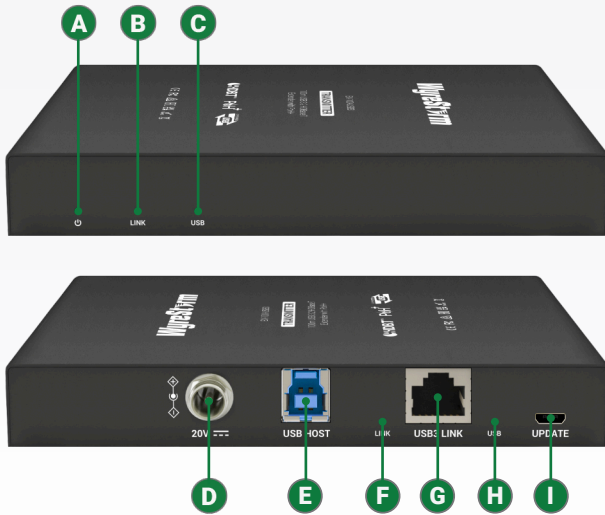
EX-100-USB3 (Front)
